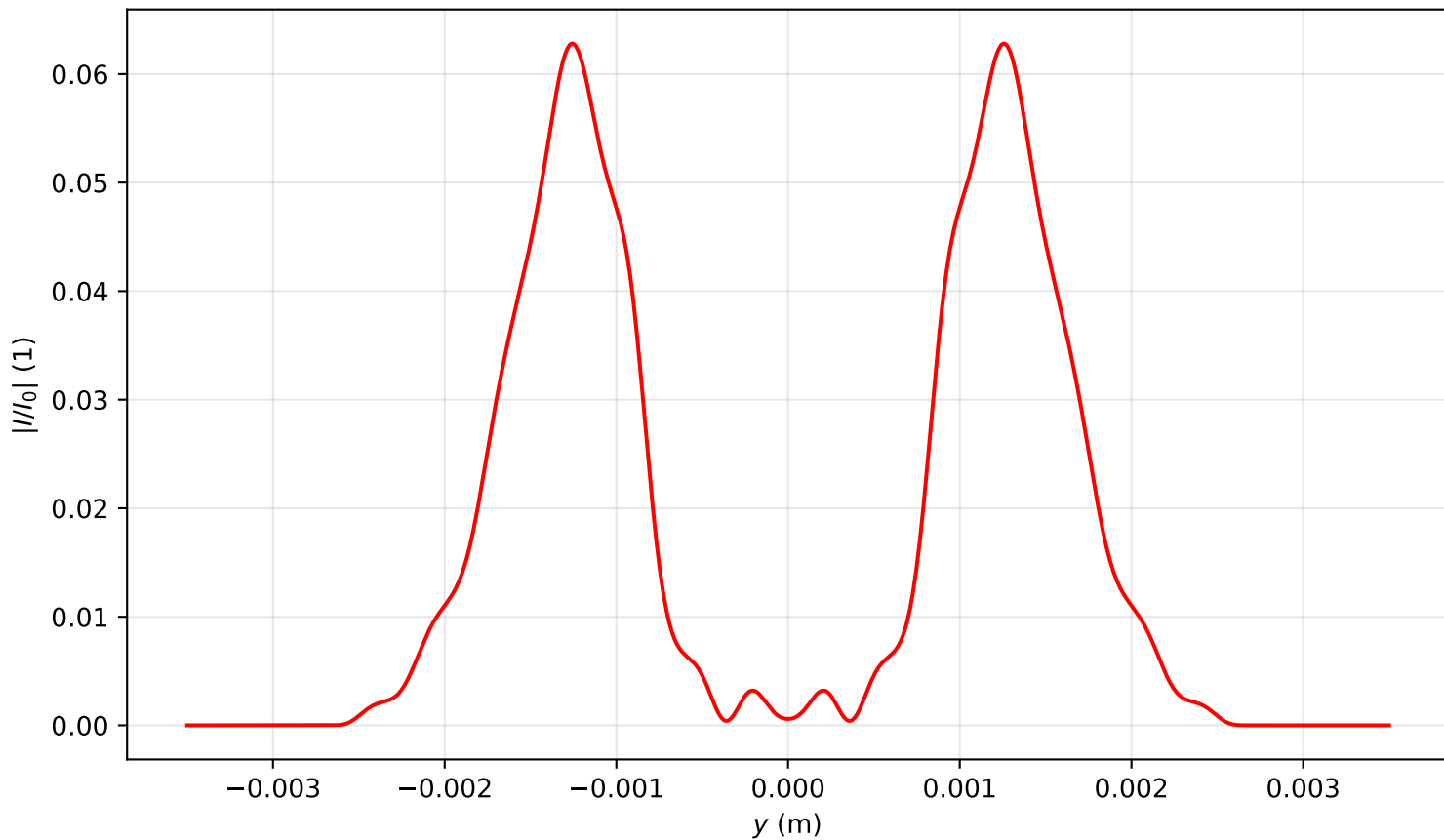
Intensity profile I(x=0, y, z=3.821)/I_0 , P_{in}=6.5P_{cr} , artificial time
